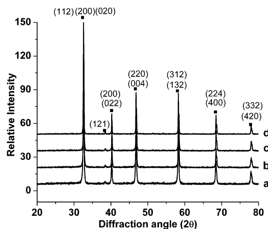
Fig. 2 X-ray diffraction patterns of \text{La}_{0.2}\text{Sr}_{0.25}\text{Ca}_{0.45}\text{TiO}_3 powders calcined in air at various temperatures: (a) 900 ^{\circ}\text{C} (S1); (b) 950 ^{\circ}\text{C} (S2); (c) 1000 ^{\circ}\text{C} (S3) and (d) 1100 ^{\circ}\text{C} (S4).
