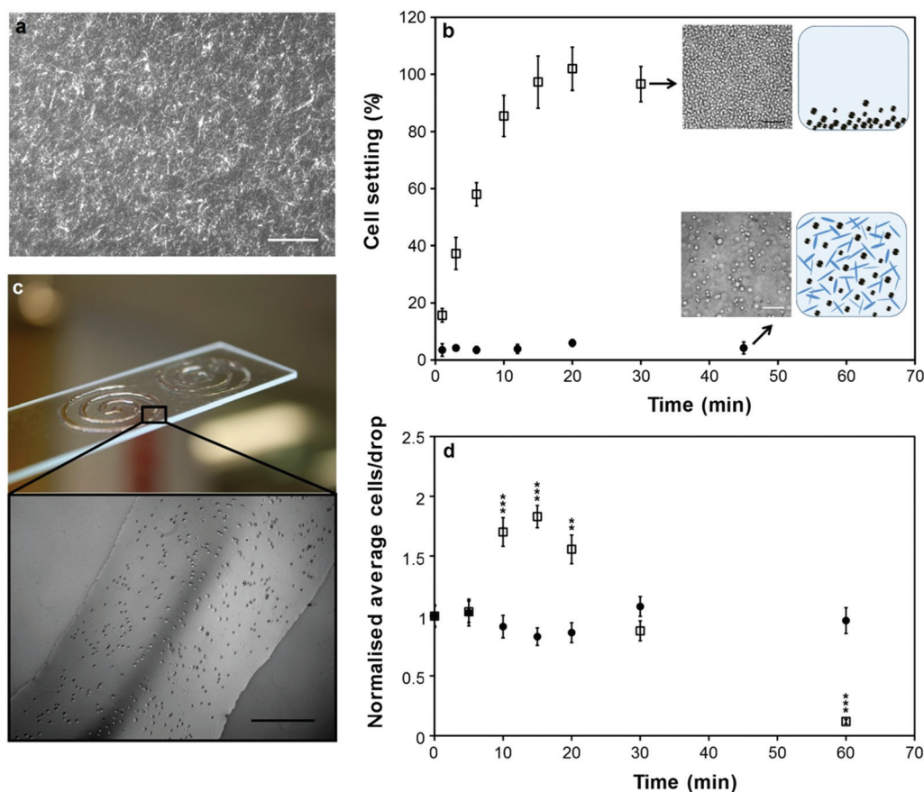
Fig. 1 Bio-ink structure and cell settling. (a) Structure of the bio-ink visualized by staining with Derivan ink and imaged by phase-contrast microscopy. Scale bar 200 μm. (b) Cell settling (percentage of cells on the base of a 96 well plate) as a function of time for C2C12 cells suspended at 1 \times 10^6 cells per mL in DMEM (open squares) or bio-ink (filled circles). Error bars represent one standard deviation from the mean. Insets show the base of well plates at indicated time points (scale bars 100 μm) and cartoons depicting the ability of the microgel suspension to keep cells in suspension. (c) Spiral patterns of C2C12 cells suspended in bio-ink and deposited on a glass slide by microvalve printing. Scale bar 500 μm. (d) Average number of cells per drop over time, normalized to the number of cells in initial drops, for C2C12 cells suspended at 2 \times 10^5 cells per mL in DMEM (open squares) or bio-ink (filled circles) and deposited by microvalve printing. Error bars represent one standard error of the mean ( n = 10 ). A statistically significant difference (compared to t = 0 min) was assessed by unpaired Student's t-test and reported with 99% (**) or 99.9% confidence (***).
