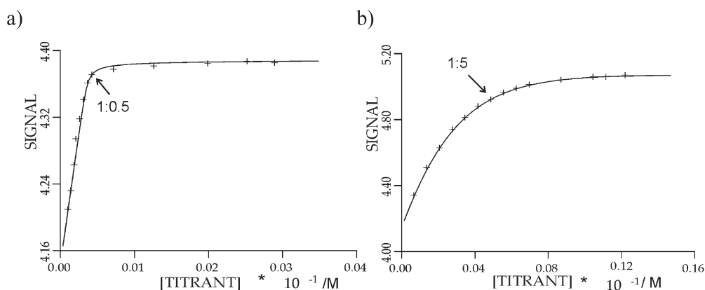
Fig. 6 Plot of the observed ( \times ) and calculated (—) chemical shifts of the NH resonances of 27 (1.02 mM) as a function of added \beta -maltoside 28 (a) or \beta -glucopyranoside 2a (b). The [receptor]:[sugar] ratio is marked. 24
