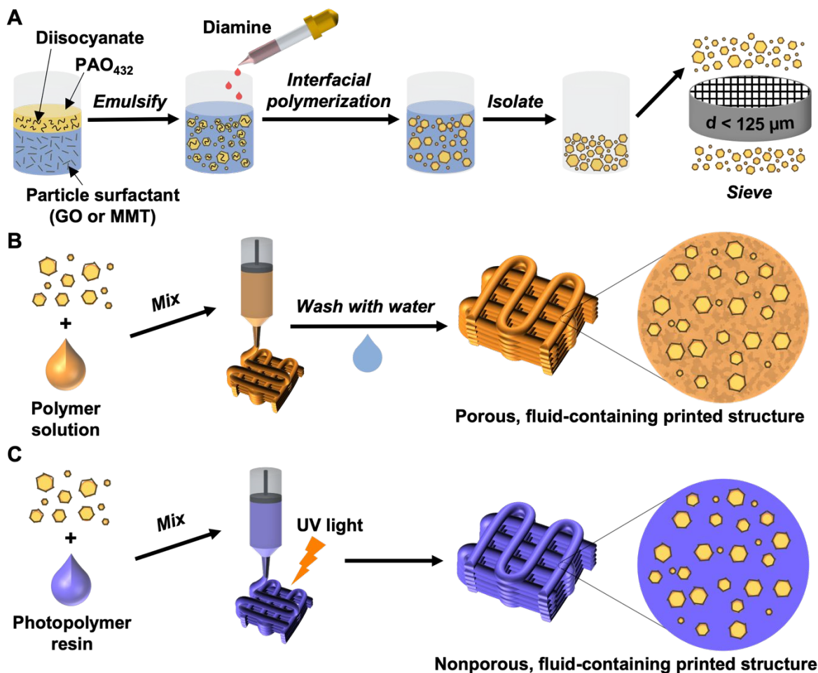
Figure 1. (A) Scheme of capsule synthesis, isolation, and sieving. (B) Combination of capsules and polymer solution, production and printing of ink, washing with water to remove solvent, and proposed porous microstructure. (C) Combination of capsules and photopolymer resin, production and printing of ink, irradiating with UV light to cure, and proposed nonporous microstructure.
