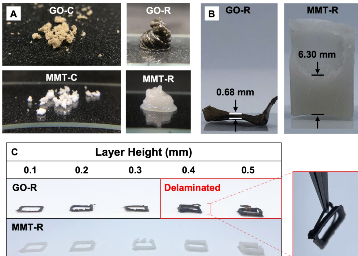
Figure 3. (A) Digital images of GO-C, GO-R, MMT-C, and MMT-R. (B) Representative samples of GO-R and MMT-R after DOC experiment, with average DOC values shown. (C) GO-R and MMT-R samples printed using different layer heights and UV cured between each layer. Image on right shows delamination of GO-R sample printed using 0.4 mm layer height.
