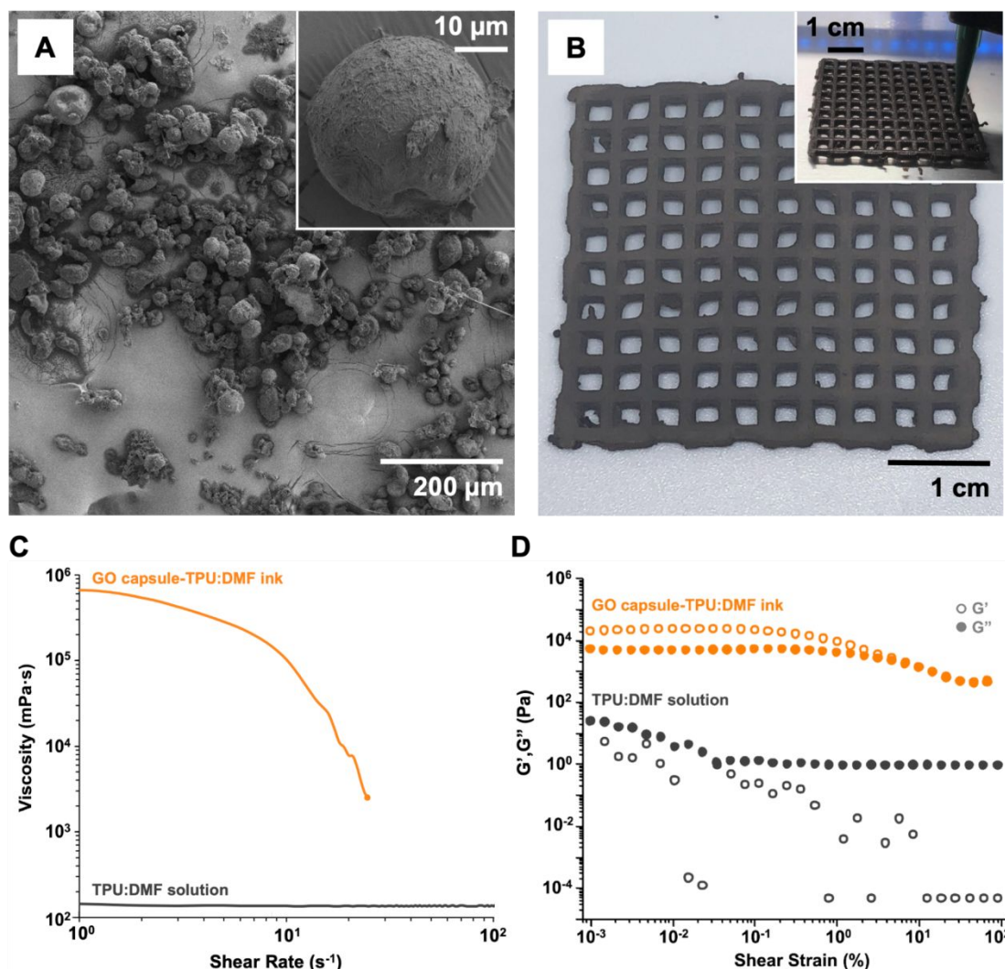
Figure 2. (A) SEM images of GO-C. (B) Printed (inset) and cured lattice prepared from GO-T ink. (C) Shear rate-dependent viscosity of TPU:DMF solution (gray trace) and GO-T (orange trace). (D) G' and G'' of TPU:DMF solution (gray markers) and GO-T (orange markers) as a function of shear strain.
