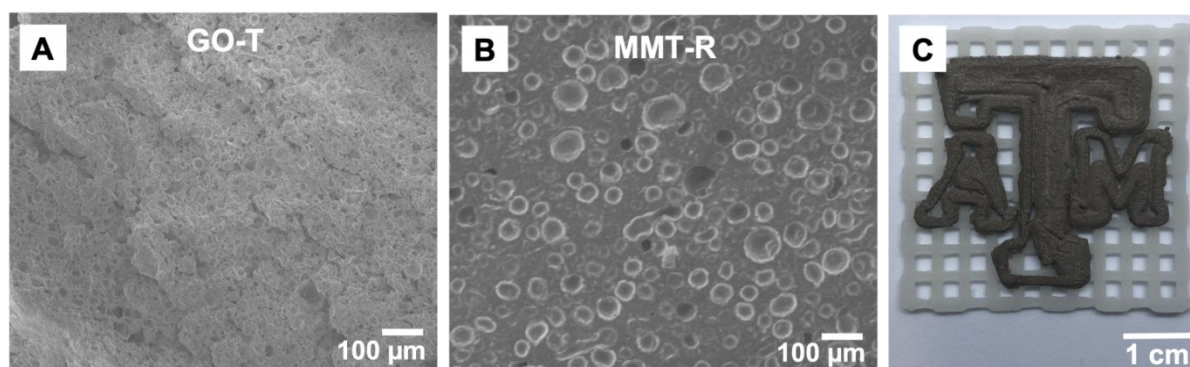
Figure 4. (A) SEM image of GO-T cross-section. (B) SEM image of MMT-R cross-section. (C) Assembled object, with lattice printed using MMT-R and Texas A&M University logo printed using GO-T.
