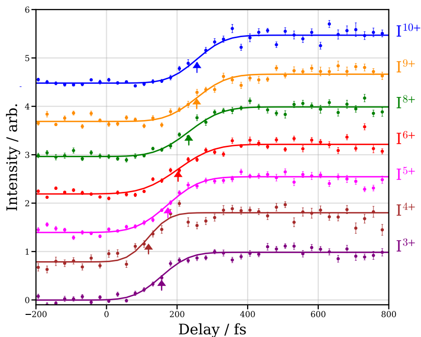
Fig. 5 Integrated ion yields as a function of pump-probe delay for Channel III for different iodine charge states, obtained by integrating the corresponding KER spectra below \sim 3.5 eV. The data are quoted with standard errors determined from a bootstrapping analysis of the dataset. The data have been fit to a Gaussian cumulative distribution function, as described in the text. The centres of the CDF fits are marked with coloured arrows.
