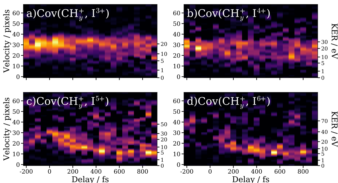
Fig. 11 Delay-dependent velocity distributions extracted from recoil-frame covariance maps between the \text{CH}_y^+ ions and \text{I}^{n+} ions with y < 3 .
