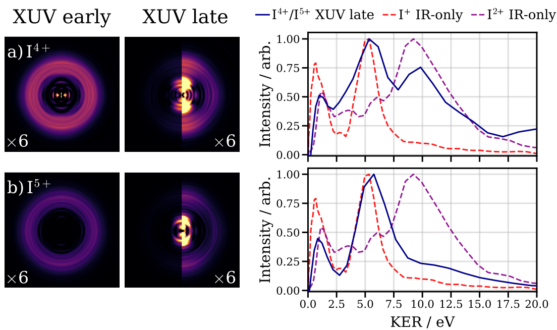
Fig. 7 Abel inverted velocity-map ion images (left) and KER distributions (right) for the (a) I^{4+} and (b) I^{5+} ions. XUV early and XUV late images are displayed, corresponding to negative and positive ( >2 ps) pump-probe delays, respectively. To increase the visibility of weak features at high KER, the intensity of the XUV early image has been multiplied by 6, as has the right hand side of the XUV late image. The IR-only KER distributions of the I^+ (red) and I^{2+} (purple) ions are plotted for comparison.
