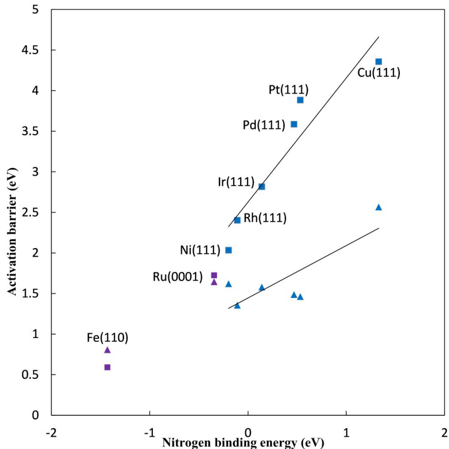
Figure 2. Activation barriers for initial N_2 activation on late transition metal surfaces at 0 V RHE, plotted against the N^* adsorption energy to the same surface. ■ - N_2 dissociation barriers, ▲ - N_2 to N_2H^* reduction barriers, blue - FCC(111) metal surfaces, purple – Fe(110) and Ru(0001) surfaces. Linear best fits are shown for FCC metals, G_{a_3} = 1.53 (N_2 \text{ binding energy}) + 2.63 \text{ eV} ( R^2 = 0.89 ) for dissociation and G_{a_1} = 0.65 (N_2 \text{ binding energy}) + 1.45 \text{ eV} ( R^2 = 0.66 ) for reduction.
