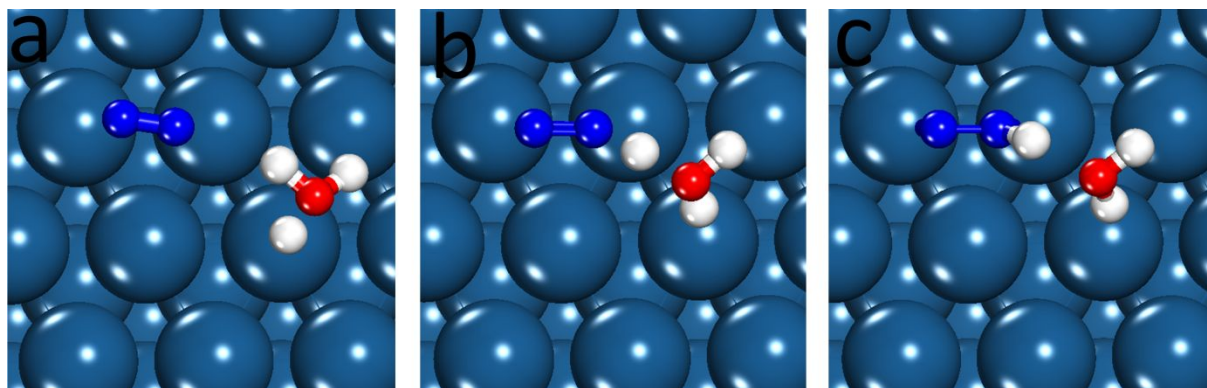
Figure 1. Equilibrium and transition states for \text{N}_2 reduction to \text{N}_2\text{H}^* on Pt(111), (a) initial state, (b) transition state and (c) final state.
