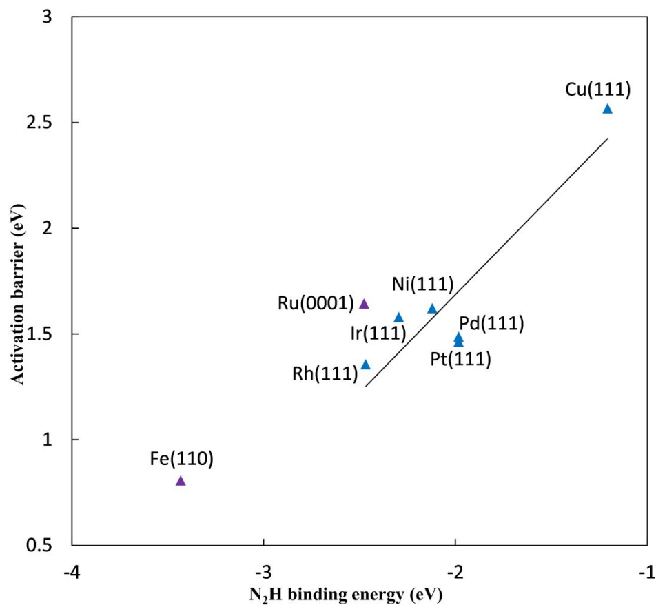
Figure 3. Activation barriers for \text{N}_2 to \text{N}_2\text{H}^* reduction on late transition metal surfaces at 0 V-RHE, plotted against \text{N}_2\text{H}^* binding energy to the same surface. Blue - FCC(111) metal surfaces, purple – Fe(110) and Ru(0001) surfaces. Linear best fit are shown for FCC metals, G_{a1} = 0.93 (\text{N}_2\text{H binding energy}) + 3.55 \text{ eV} ( R^2 = 0.83 ).
