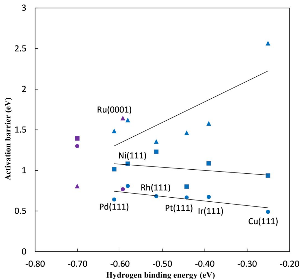
Figure 6. Activation barriers for \text{N}_2 and \text{NH}^* reduction and hydrogen evolution on late transition metal surfaces at 0 V-RHE, plotted against hydrogen binding energy to the same surface. \blacktriangle - \text{N}_2 to \text{N}_2\text{H}^* reduction barriers, \blacksquare - \text{NH}^* to \text{NH}_2^* reduction barriers, \bullet - HER barriers, blue - FCC(111) metal surfaces, purple - Fe(110) and Ru(0001) surfaces. Linear best fit are shown for FCC metals, G_{a_1} = 2.54(\text{Hydrogen binding energy}) + 2.86 \text{ eV} ( R^2 = 0.59 ) for \text{N}_2 reduction, G_{a_2} = -0.38(\text{Hydrogen binding energy}) + 0.85 \text{ eV} ( R^2 = 0.12 ) for \text{NH}^* reduction and G_{a_{\text{H}_2}} = -0.56(\text{Hydrogen binding energy}) + 0.40 \text{ eV} ( R^2 = 0.55 ) for HER.
