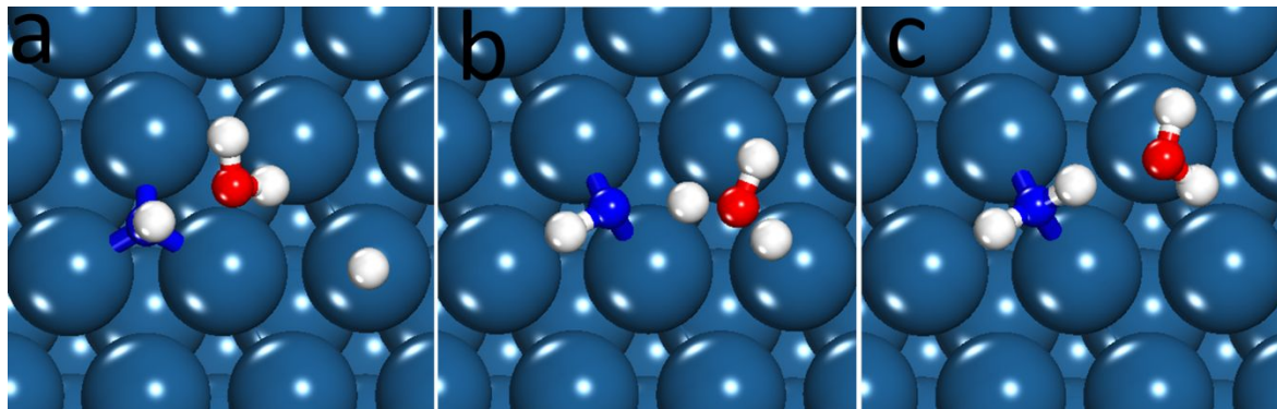
Figure 4. Reaction path for \text{NH}^* hydrogenation on the Pt(111) surface, (a) initial state, (b) transition state and (c) final state
