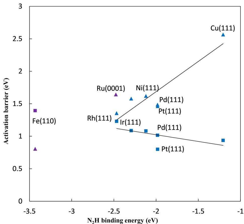
Figure 5. Activation barriers for N_2 and NH^* reduction on late transition metal surfaces at 0 V-RHE, plotted against N_2H^* binding energy to the same surface. \blacktriangle - N_2 to N_2H^* reduction barriers, \blacksquare - NH^* to NH_2^* reduction barriers, blue - FCC(111) metal surfaces, purple - Fe(110) and Ru(0001) surfaces. Linear best fit are shown for fcc metals, G_{a1} = 0.93(N_2H^* \text{ binding energy}) + 3.55 \text{ eV} ( R^2 = 0.83 ) for N_2 reduction and G_{a2} = -0.21(N_2H^* \text{ binding energy}) + 0.61 \text{ eV} ( R^2 = 0.37 ) for NH^* reduction.
