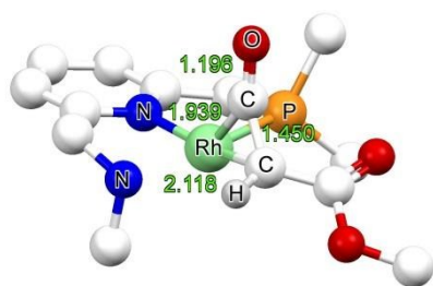
Fig. 3. DFT optimized structure of ^{N}INT3 (Bond length in Å).
