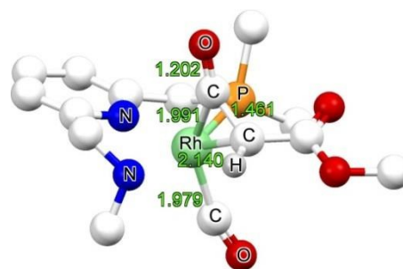
Fig. 4. DFT optimized structure of ^{N}INT6 (Bond length in Å).
