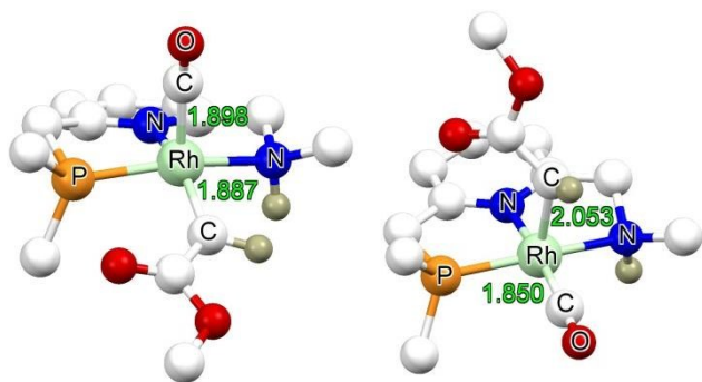
Fig. 2. DFT optimized structure of, Left: ^{NH}INT2^b , Right: ^{NH}INT2^a (Bond length in Å).
