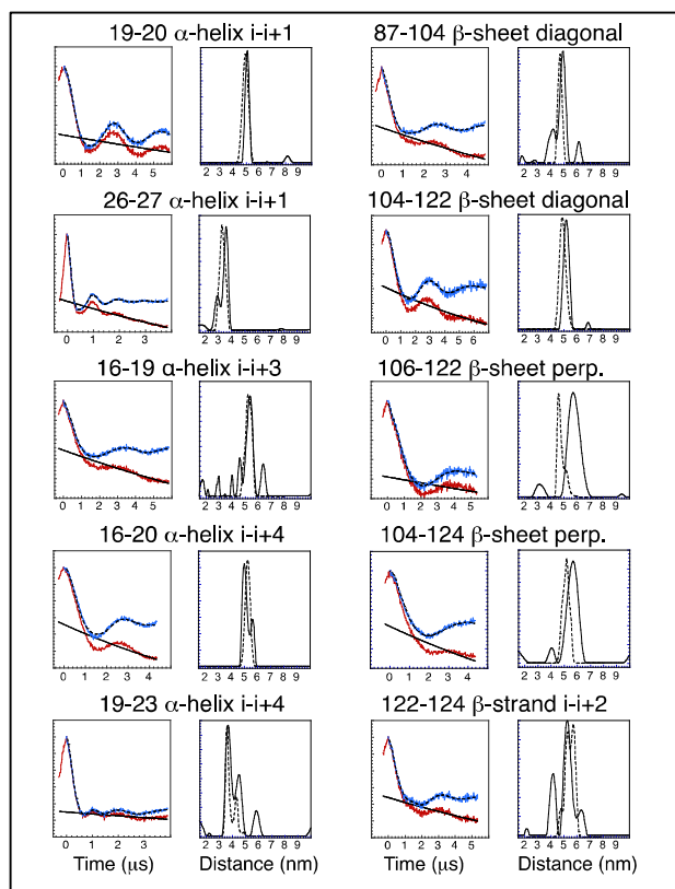
Fig. 3 Diagram showing plots of X-band PELDOR data, uncorrected (red) and background corrected (blue) next to distance distributions calculated by Tikhonov regularization (solid black line) and predicted distributions from dynamic simulations (dashed line).
