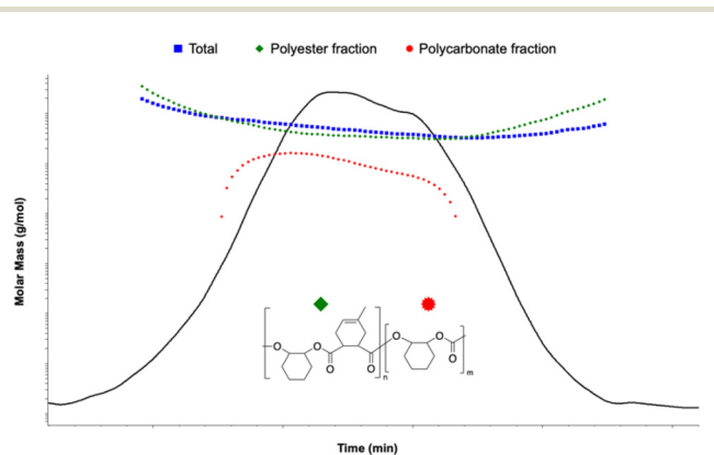
Fig. 8 GPC light scattering trace demonstrating molecular weight fractions of polyester- block -polycarbonate (Table 2, entry 3). Fractions determined via ASTRA software (Wyatt) GPC conjugate analysis method.
