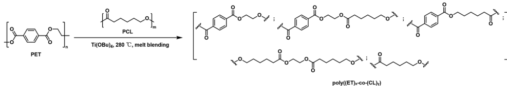
Fig. 10 Synthesis of poly((ET) x -co-(CL) y ) via transesterification of PET and PCL through melt blending.
