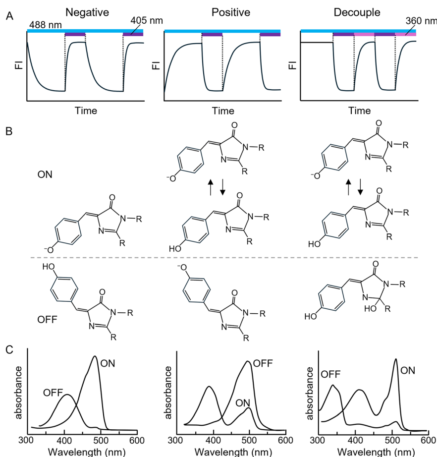
Fig. 2 Photoswitching of GFP-like rsFP. (A) Fluorescence response of GFP-like green n -rsFPs (left), green p -rsFPs (middle), and decouple type rsFPs (right) to continuous irradiation at 488 nm and intermittent irradiation at 405 nm and/or 360 nm. (B) Chromophore isomerisation, hydration, and protonation states in the ON and OFF states of n -rsFPs (left), green p -rsFPs (middle), and decouple type green rsFPs (right). (C) Illustration of absorbance spectra in the ON and OFF states of n -rsFPs (left), green p -rsFPs (middle), and decouple type green rsFPs (right).
