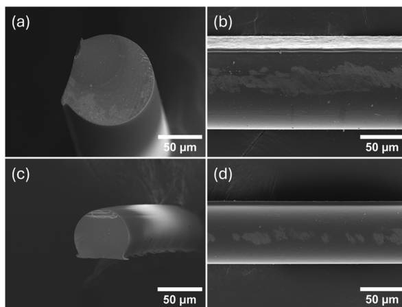
Fig. 1 SEM images of air-dried as-spun Kraft lignin–PVA fibres spun continuously from [DMBA][HSO 4 ] and water mixtures using a 25 G (260 \mu m) spinneret (a and b) and a 30 G (159 \mu m) spinneret (c and d).
