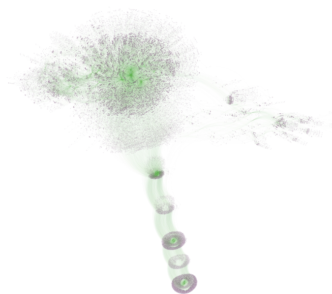
Fig. 1 A segment of the AiiDA database spanning this screening is depicted, showcasing a small subset pertaining to single-point calculations performed on approximately 1500 structures at the level of DFT. Purple nodes represent either data instances (i.e., inputs and outputs of calculations) or the calculations themselves, while green links illustrate the logical provenance connecting these nodes.
