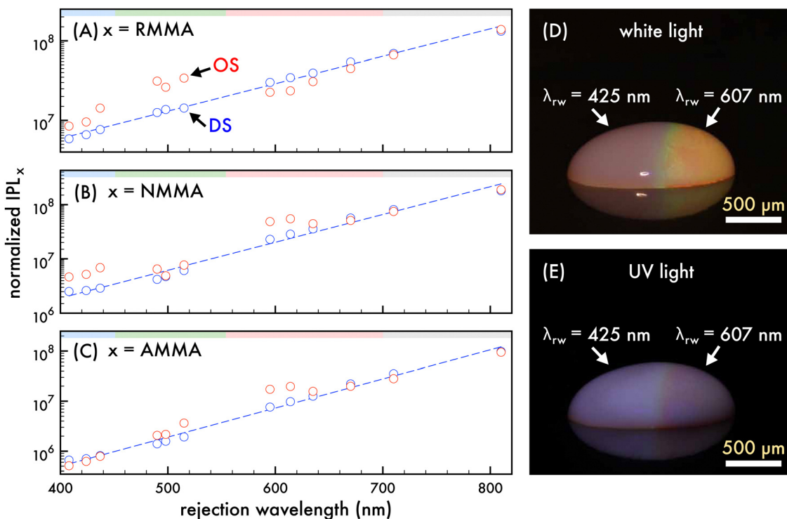
Fig. 2 Comparison of the integrated photoluminescence of n_1 assembled in an ordered structure and corresponding disordered structure with dilution. Normalized integrated photoluminescence ( IPL ) of the n_1 ordered structure (OS, red circles) and disordered structure (DS, blue circles) emission attributed to (A) RMMA, (B) NMMA, and (C) AMMA as the rejection wavelength ( \lambda_{rw} ) of the OS was shifted through the visible spectrum by dilution with deionized water. A 370 nm excitation wavelength was utilized to obtain PL spectra presented in (A) – (C) and the IPL was normalized by the concentration of nanoparticles in each dilution. The spectral regions attributed to AMMA (blue), NMMA (green), RMMA (red) emission are lightly shaded at the top of (A) – (C) as a visual aid. A trendline for the DS IPL (blue dashed line) is included in (A) – (C) to aid the eye. Photographs of a ca. 500 \mu L droplet the n_1 OS under (D) white light and (E) UV light exposure, where the \lambda_{rw} of the left and right half of the OS droplet was at 425 nm and 607 nm, respectively. Scale bars are approximate.
