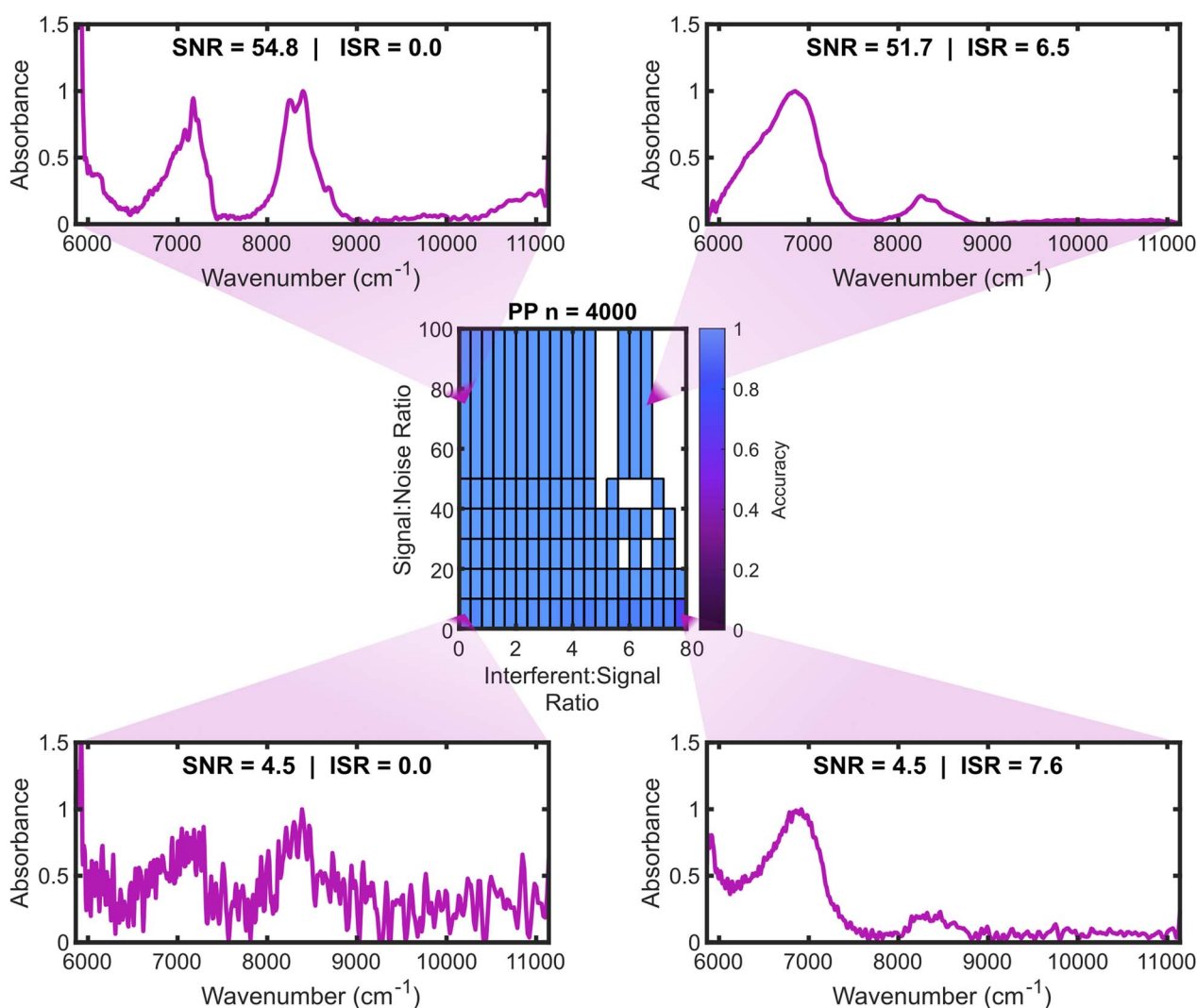
Fig. 6 Two-dimensional histogram tiles illustrating the performance of the cubic SVM model trained on spectral data augmented with both noise and interferences for polypropylene. Signal-to-noise ratios (SNR) are shown on the y-axis, interferent-to-signal ratios (ISR) on the x-axis, and accuracy is depicted by the color scale. White regions indicate areas without data. A sample spectrum from each quadrant of the plot is included, with frequency ( \text{cm}^{-1} ) on the x-axis and absorbance on the y-axis. As SNR decreases, spectral features become increasingly unclear by noise, while higher ISR values reflect greater overlap of spectral features by those of water and plant matter.
