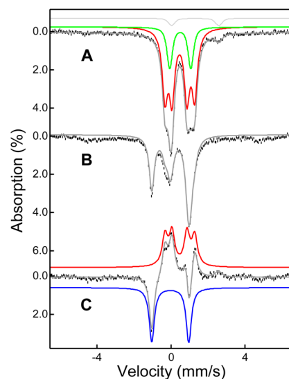
Fig. 4 4.2 K zero field Mössbauer spectra (vertical bars) of 2+\text{Sc} (panel A) and upon conversion of 2+\text{Sc} into 3 (panel B). Panel C shows the B – A difference spectrum highlighting the conversion of 2+\text{Sc} to 3 . Panel A shows an overall simulation (grey solid line) with four species. The red solid line containing two distinct ferric doublets of equal intensity represents 74% of the iron in the sample and is assigned to the dominant 2+\text{Sc} species with distinct \text{Fe}^{\text{III}} units. The green solid line represents 18% of the iron in the sample corresponding to a symmetric diferric species. The light grey line represents a minor ferrous species (~5%), likely to be the starting ferrous complex. Panel B shows an overall simulation (grey solid line) with 50% 3 , 25% 2+\text{Sc} and 18% 2' . Panel C shows the conversion of 2+\text{Sc} (red solid line) into 3 (blue solid line).
