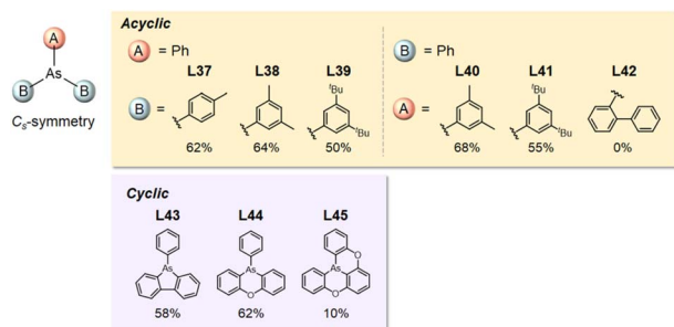
Fig. 5 o -, m -, and p -substituted C_5 -type arse ligands. NMR yields are shown below the structures.
