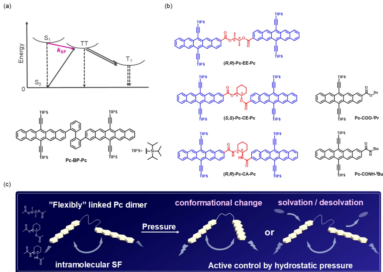
Fig. 1 (a) (Top) schematic diagram of SF in a TIPS-modified pentacene (Pc) dimer: k_{\text{SF}} represents the rate constant of SF from S_1 to TT; in the present Pc case, the reverse triplet–triplet annihilation (TTA) can be omitted, due to the large exergonic reaction (ca. 0.3 eV). 45 (Bottom) chemical structure of Pc-BP-Pc. (b) Chemical structures of SF-active dimers; (R,R)-Pc-EE-Pc, (S,S)-Pc-CE-Pc, and (R,R)-Pc-CA-Pc, the corresponding referenced monomers; Pc-COO- i Pr and Pc-CONH- i Bu. (c) Conceptual illustration of active control of SF-active soft materials driven by hydrostatic pressure.
