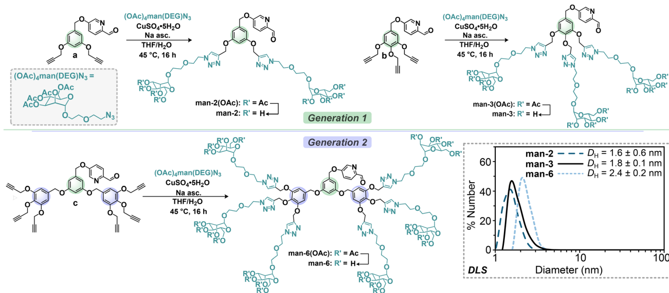
Fig. 2 Synthetic schemes for the preparation of dendritic subcomponents man-2 , man-3 , and man-6 from a , b , and c precursors, respectively, with corresponding DLS data (bottom right, measured in H 2 O, 1 mM).
