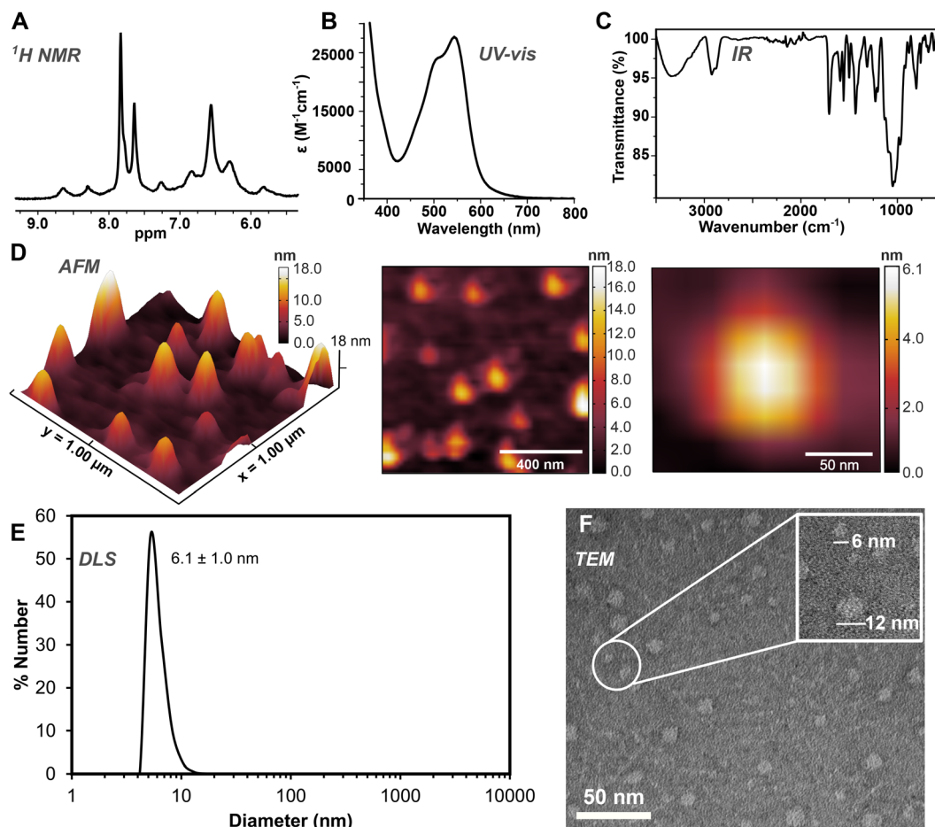
Fig. 3 Characterization data of [3][\text{BF}_4]_8 : (A) ^1\text{H} NMR spectrum ( \text{D}_2\text{O} , 45 ^\circ\text{C} ); (B) UV-vis spectrum ( \text{H}_2\text{O} , 50 \mu\text{M} ); (C) ATR-IR spectrum; (D) AFM images and height profiles (tapping mode, air, 298 K) of a drop-cast \text{H}_2\text{O} solution (0.2 \mu\text{M} ) on mica; (E) DLS measurement (50 \mu\text{M} , 85% v/v DMSO/ \text{H}_2\text{O} ); (F) negative-contrast electron micrograph (uranyl acetate).
