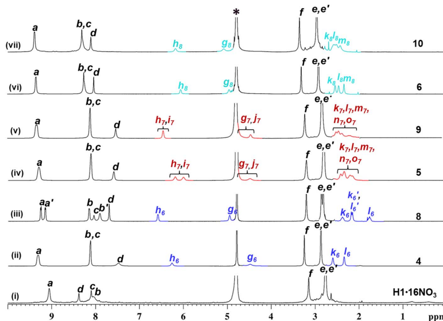
Fig. 6 ^1\text{H} NMR spectra (400 MHz, \text{D}_2\text{O} , 298 K, i.e., 25 ^\circ\text{C} ) for isolated samples of (i) \text{H1}\cdot 16\text{NO}_3 , (ii) [(\text{H6})_2 < \text{H1}]\cdot 16\text{NO}_3 (4), (iii) [\{\text{G} < (\text{H6})_2\} < \text{H1}]\cdot 17\text{NO}_3 (8), (iv) [(\text{H7})_2 < \text{H1}]\cdot 16\text{NO}_3 (5), (v) [\{\text{G} < (\text{H7})_2\} < \text{H1}]\cdot 17\text{NO}_3 (9), (vi) [(\text{H8})_2 < \text{H1}]\cdot 16\text{NO}_3 (6), and (vii) [\{\text{G} < (\text{H8})_2\} < \text{H1}]\cdot 17\text{NO}_3 (10).
