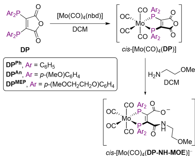
Scheme 2 Mo(0) complexation of DP ligands to give \text{cis-[Mo(CO)}_4\text{(DP)]} and subsequent ring-opening to give \text{cis-[Mo(CO)}_4\text{(DP-NH-MOE)]}^- .
