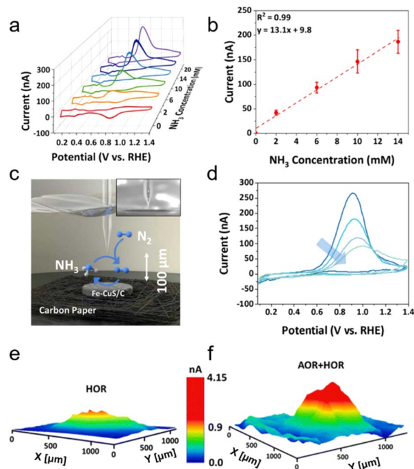
Fig. 3 (a) CVs of \text{NH}_3 oxidation at the modified Pt UME in 1 \text{ M KOH} solution containing 0 to 20 \text{ mM NH}_3 . Scan rate: 20 \text{ mV s}^{-1} . (b) The relationship between \text{NH}_3 concentration and the peak current of the AOR in 1 \text{ M KOH} solution. (c) A schematic diagram of the study of the NRR on the Fe-CuS/C-loaded carbon paper with a Pt UME in the SECM SG-TC mode. The inset shows an actual image of the experimental setup. (d) Repetitive CVs of the AOR were collected at the Pt UME when the UME was positioned close to the Fe-CuS/C-loaded carbon paper. The carbon paper was biased at -0.2 \text{ V vs. RHE} . Scan rate: 20 \text{ mV s}^{-1} . Reproduced with permission from ref. 93, Elsevier, 2023. (e and f) Three-dimensional SECM image showing the local catalytic activity of Cu-Ni 4 B 3 (1:2). The tip was biased at a potential of 1.1 \text{ V} in (e) under an Ar atmosphere to quantify the HOR on the tip, and in (f) under a \text{N}_2 atmosphere to detect the products of both the HER and NRR. Reproduced with permission from ref. 95, Royal Society of Chemistry, 2023.
