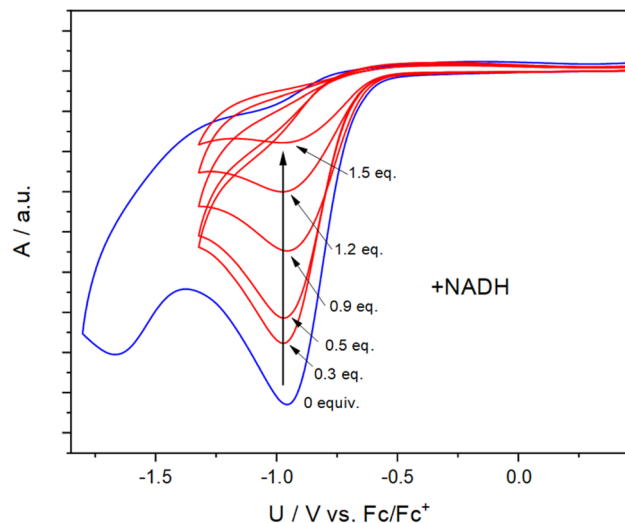
Fig. 3 Cyclovoltammogram of 1c (blue curve, 30 mM concentration, solvent: MeCN, scan rate: 500 mV s -1 , supporting salt: Bu 4 NClO 4 (0.1 M), working electrode: Pt). The red curves indicate the decrease of the reduction peak upon addition of NADH.
