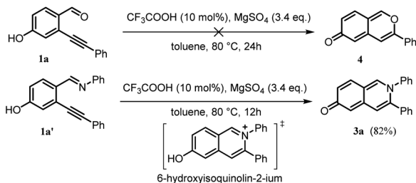
Scheme 3 Control experiments.
