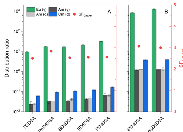
Fig. 6 Distribution ratios for stripping of Eu, Am, and Cm with \text{SO}_3\text{-Ph-BTBP} . Organic phase: 0.1 \text{ mol L}^{-1} diglycolamide extractant dissolved in n -dodecane + 5 vol% 1-octanol, loaded from a solution containing 18 \text{ mmol L}^{-1} \text{Ln(III)} (A) or 10^{-5} \text{ mol L}^{-1} \text{Eu(III)} (B) + 50 \text{ kBq mL}^{-1} of ^{152}\text{Eu} , ^{241}\text{Am} , and ^{244}\text{Cm} each dissolved in 3 \text{ mol L}^{-1} \text{HNO}_3 solution. Aqueous phase: 10 \text{ mmol L}^{-1} \text{SO}_3\text{-Ph-BTBP} dissolved in 0.3 \text{ mol L}^{-1} \text{HNO}_3 solution. Shaking time: 30 min. Temperature: 20^\circ\text{C} .
