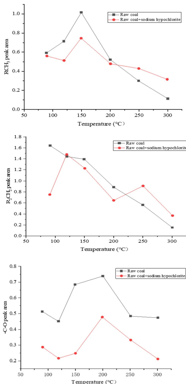
Fig. 5 Changing curve of peak absorption area of \text{RCH}_3 and \text{R}_2\text{CH}_2 and -\text{C}=\text{O} group and temperature.
