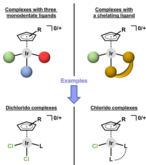
Fig. 3 Two basic structural types of half-sandwich iridium(III) cyclopentadienyl complexes ( \text{Ir}-\text{Cp}^{\text{x}} ).
