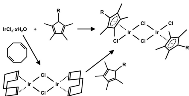
Scheme 1 Synthesis of the most used dinuclear intermediate, [\text{Ir}(\mu\text{-Cl})(\eta^5\text{-Cp}^{\text{x}})\text{Cl}]_2 , for the synthesis of half-sandwich Ir(III) cyclopentadienyl complexes.
