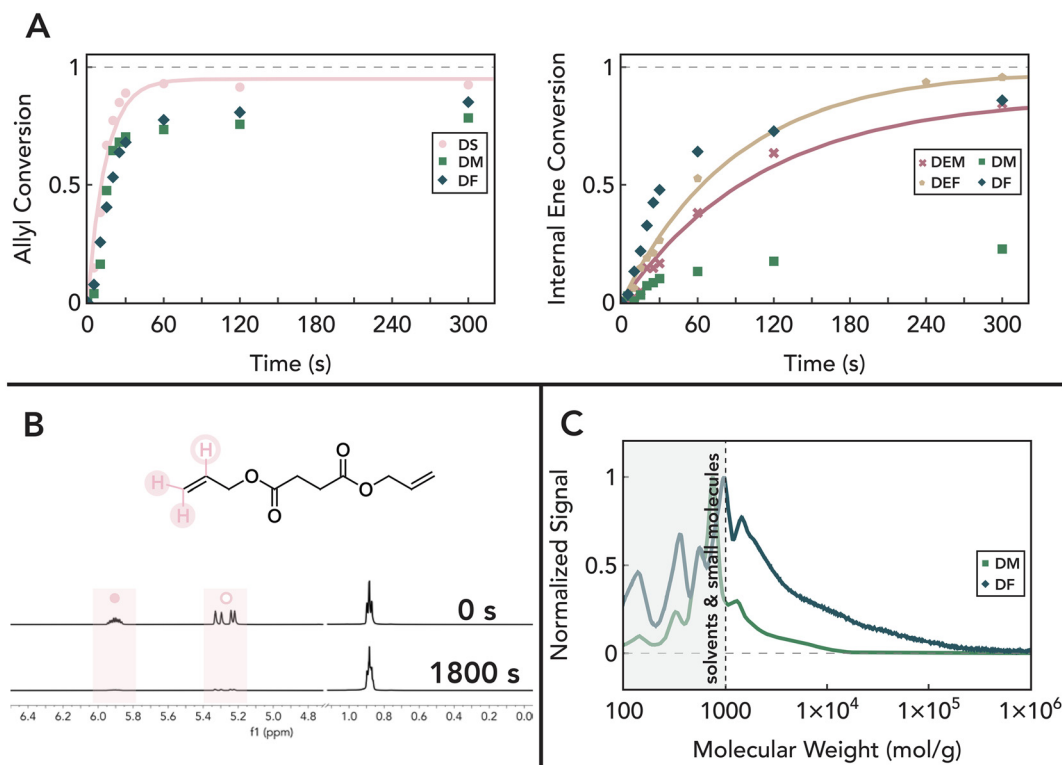
Fig. 2 (A) ^1\text{H} NMR conversion of allyl (left) and maleate/fumarate (right) functional groups in 1:1 ratio* photoreactions shows that consumption of maleate/fumarate groups occurs along with thiol addition to allyl ethers. The solid-line fits to first order kinetics are shown for pure thiol-ene mechanisms and omitted for others for clarity; see the ESI† for other fits. (B) The extent of photoreaction is monitored via integration of characteristic peaks of the ^1\text{H} NMR spectra, as shown here for DS used in a 1:1 ratio* photoreaction from 0–1800 s. Peaks corresponding to the terminal carbon of 1-hexanethiol was used for normalization. (C) SEC traces of 1:1 ratio* photoreactions of DM and DF after 30 minutes reveal formation of higher molecular-weight adducts, suggesting homopolymerization of maleate/fumarate groups. Molecular weights are estimates determined from polystyrene standards. *The ratio is allyl : thiol or fumarate/maleate : thiol for DEF and DEM.
