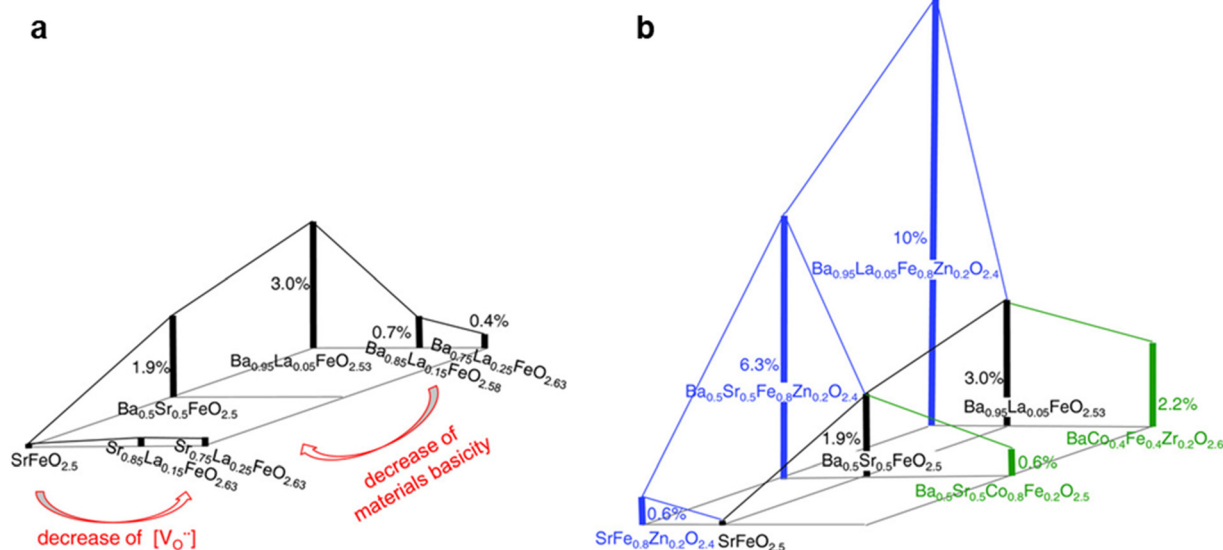
Fig. 8 Proton concentration in perovskite oxides systems of (Ba, Sr, La)(Fe, Co, Zn)O 3-δ system at 250 °C and 16 mbar H 2 O. (a) Effect of A-site cations (Ba, Sr and La) and (b) effect of B-site cations (Fe, Co and Zn). This figure has been adapted from ref. with permission from John Wiley & Sons, copyright 2025.
