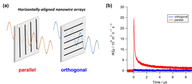
Fig. 4 Non-contact electrical conduction measurement of nanowires by TRMC method. (a) Schematic illustration of anisotropic conduction measurement of the nanowire under polarized light. (b) FP-TRMC profiles ( \lambda_{\text{ex}} = 355 \text{ nm} ; photon intensity = 10 \text{ mJ cm}^{-2} ) of \text{C}_{60} nanowire arrays (red: parallel; blue: orthogonal). The inset illustration represents TRMC measurement for horizontally aligned nanowire arrays. Polarized microwaves were injected with electric field oscillation directions parallel or perpendicular along the nanowire arrays. These measurements were fixed for f = 1 \times 10^{11} \text{ cm}^{-2} .
