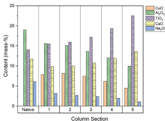
Fig. 12 Metal oxide distribution in the column after adsorption by XRF. The concentration of copper solution after 31 adsorption-desorption cycles was 1000 \text{ mg L}^{-1} , pH was 4.5 and temperature 25^\circ\text{C} . Fresh adsorbent is labeled as native for comparison.
