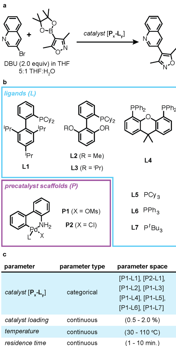
Fig. 5 (a) Reaction scheme for the Suzuki–Miyaura cross-coupling of 3-bromoquinoline with 3,5-dimethylisoxazole-4-boronic acid pinacol ester in the presence of 1,8-diaza-bicyclo[5.4.0]undec-7-ene (DBU) and THF/water. (b) The precatalyst scaffolds (P) and ligands (L) that comprise the catalysts explored in this study. (c) The optimisation space for this case study is composed of four parameters.
