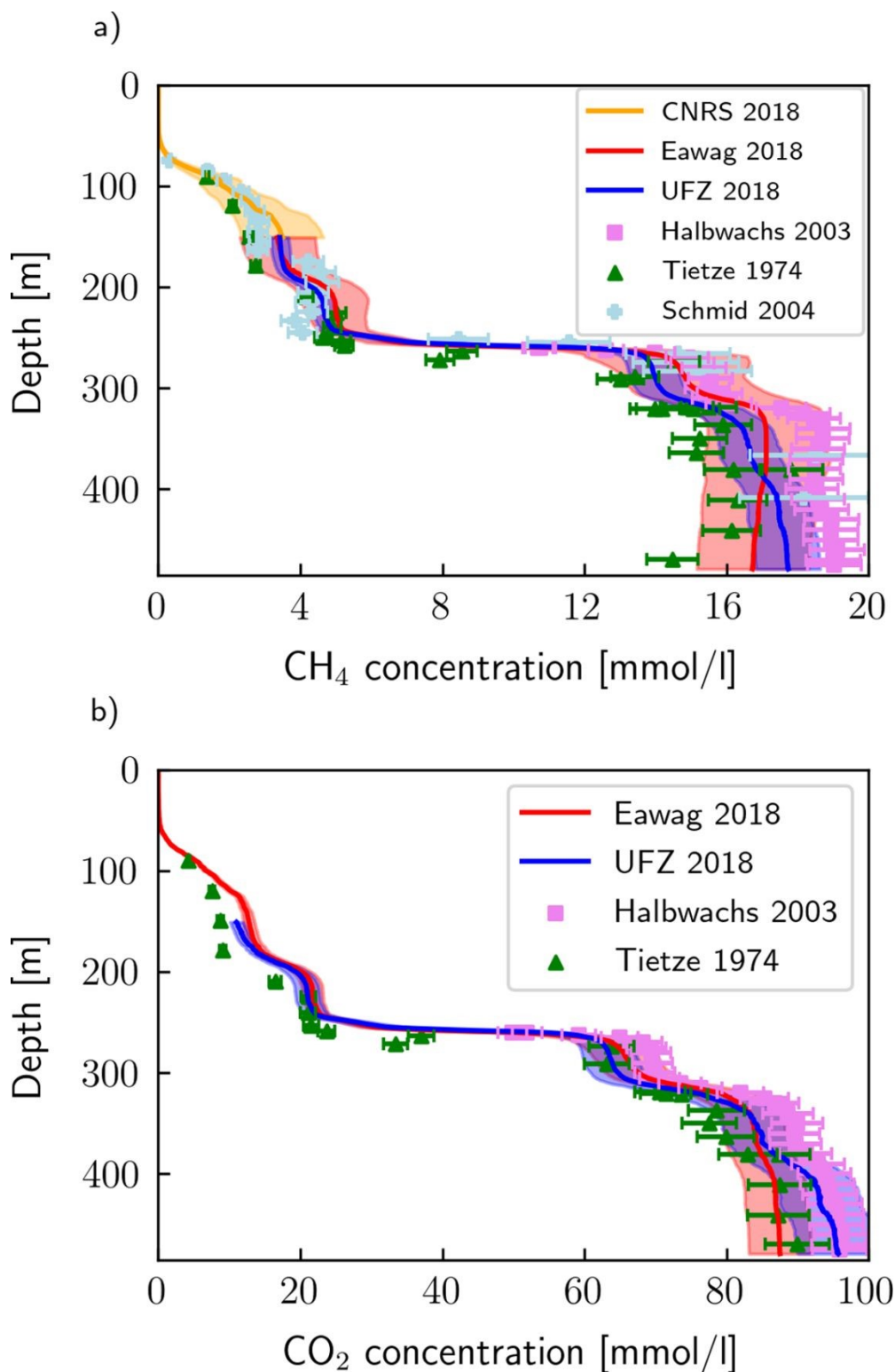
Fig. 3: Comparison between dissolved \text{CH}_4 and \text{CO}_2 concentrations measured by the 2018 campaign and those measured in 1974, 2003, and 2004. Reprinted (adapted) from reference 24. Copyright 2020 The Authors. 24
