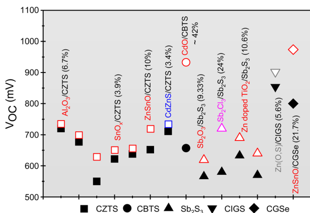
Fig. 11 V_{\text{oc}} improvements observed in proven and emerging material-based SCs with various passivation layers. Hollow symbols represent V_{\text{oc}} without passivation layers, while filled symbols indicate V_{\text{oc}} with passivation layers. Colors denote different passivation types: Red for oxide-based, Blue for sulfur-based, Pink for chlorine-based, and Gray for oxy-sulfide-based layers.
