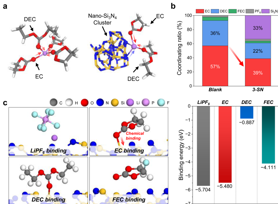
Fig. 3 Theoretical investigation of influence of the nano- \text{Si}_3\text{N}_4 on \text{Li}^+ solvation environment. (a)–(c) Solvation and interaction characteristics of the electrolyte and nano- \text{Si}_3\text{N}_4 . (a) Coordinated structures around \text{Li}^+ in the Blank and 3-SN. (b) The ratio of electrolytes coordinated with \text{Li}^+ according to the Blank and 3-SN. (c) Interaction characteristics of \text{LiPF}_6 , EC, DEC, and FEC on the \alpha\text{-Si}_3\text{N}_4 (101) surface.
