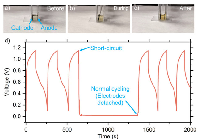
Fig. 6 Test setup with a cathode and an anode in the electrolyte (~590 μL) with three different electrode configurations (a) before, (b) during, and (c) after the short circuit, and (d) corresponding voltage profile against time.
