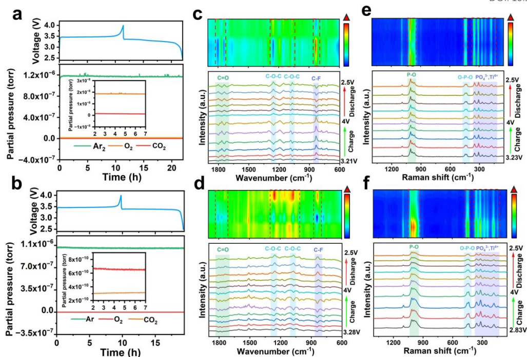
Fig. 6 In-situ characterization of the interaction mechanism of the PGPE@P-LATP10-J composite layer. Voltage profile and corresponding in situ DEMS results of various mass signals (a) PGPE@P-LATP10-J and (b) PGPE@P-LATP10, respectively. In situ FT-IR spectra and the corresponding contour mapping of (c) PGPE@P-LATP10-J and (d) PGPE@P-LATP10, respectively. In situ Raman spectra and the corresponding contour mapping of (e) PGPE@P-LATP10-J and (f) PGPE@P-LATP10, respectively.
