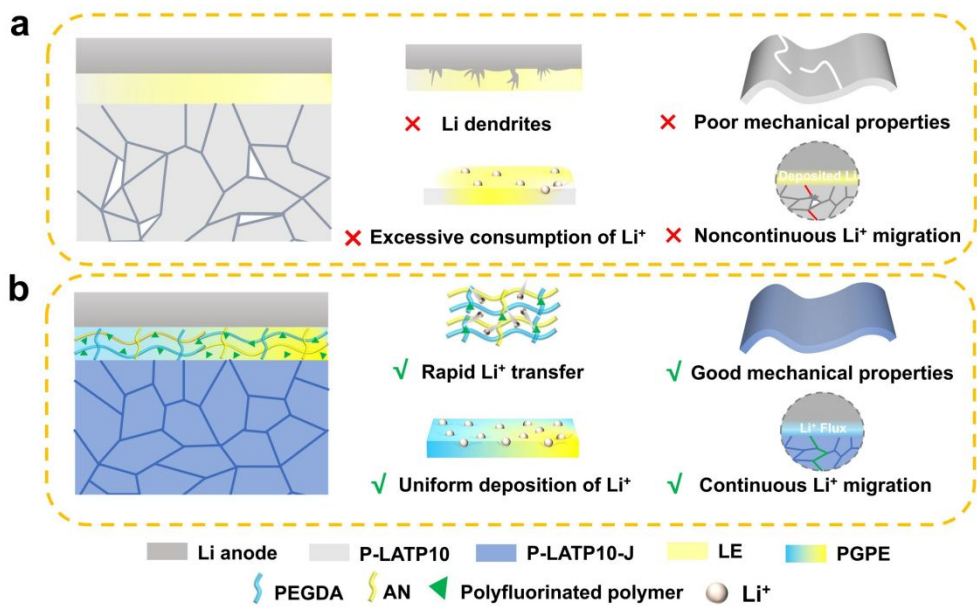
Fig. 1 Schematic illustrations of Li/LATP interfacial. Comparative analysis for advantages of (a) P-LATP as compared with (b) PGPE@P-LATP-J.
