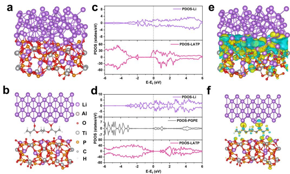
Fig. 7 (a) and (b) the interface model structures of Li/LATP and Li/PGPE/LATP, respectively. (c) and (d) the PDOS of Li/LATP and Li/PGPE/LATP, respectively. (e) and (f) the charge density difference of Li/LATP and Li/PGPE/LATP, respectively.
