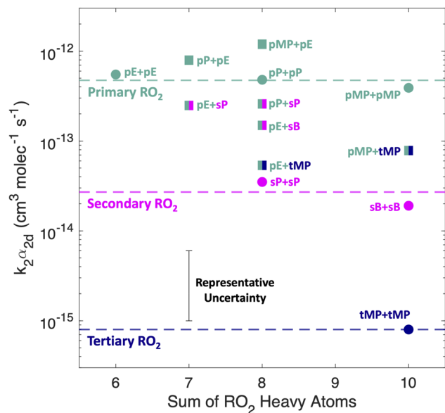
Fig. 4 Measured values of k_{2\alpha_{2d}} for the self-reactions of the ethene, methylpropene, propene, and cis -2-butene-derived peroxy radical systems, plotted as a function of the sum of the number of heavy atoms in the participating peroxy radicals and colored by substitution of the peroxy radical. Dashed lines give the average value of k_{2\alpha_{2d}} for each of the primary, secondary, and tertiary peroxy radical groups. Squares give k_{2\alpha_{2d}} values for the cross-reactions measured in this work. All points are labeled with the participating peroxy radicals.
