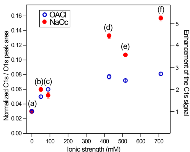
Fig. 6 Normalized C 1s/O 1s ratio vs. ionic strength of accompanying negatively charged NaOc ( \text{Na}^+ + \text{C}_7\text{H}_{15}\text{COO}^- ) and positively charged OAcI ( \text{C}_7\text{H}_{15}\text{CHN}_3^+ + \text{Cl}^- ) surfactants in the presence of different salts. (a) Pure water, (b) 50 mM NaCl, (c) 29 mM \text{Na}_2\text{SO}_4 , (d) 426 mM NaCl, (e) 29 mM \text{Na}_2\text{SO}_4 + 426 mM NaCl, and (f) 520 mM ASW. The error bars indicate the variation from the average of two data points.
