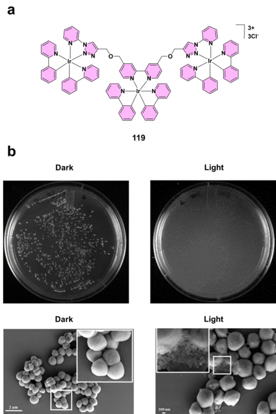
Fig. 14 (a) Structure of complex 119. (b) Upper panel: impact on the viability of MRSA (as measured by colony-forming units, CFU) following treatment with complex 119, with and without photoirradiation. Without photoirradiation, complex 119 ( 25 \mu\text{g mL}^{-1} ) showed no significant effect on MRSA viability, confirming its “bacteria-safe” property. However, under photoirradiation, complex 119 ( 25 \mu\text{g mL}^{-1} ) caused a marked reduction in MRSA, demonstrating a positive photodynamic therapy (PDT) effect. Representative images of MRSA colonies post-treatment with complex 119 ( 25 \mu\text{g mL}^{-1} ) with or without photoirradiation are shown. All error bars represent the standard error of the mean (mean \pm SEM) ( n = 6 ) from two biological replicates. Lower panel: MRSA cells exhibited no significant morphological changes when treated with complex 119 ( 25 \mu\text{g mL}^{-1} ) without photoirradiation, but clear cellular damage was observed when photoirradiation was applied, indicating a successful PDT effect. Reproduced from ref. 71 with permission from Wiley-VCH, copyright 2024.
