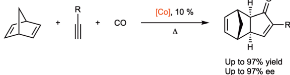
Scheme 33 Intermolecular PK catalyzed by Co-ThaxPHOS (L75–L77).
