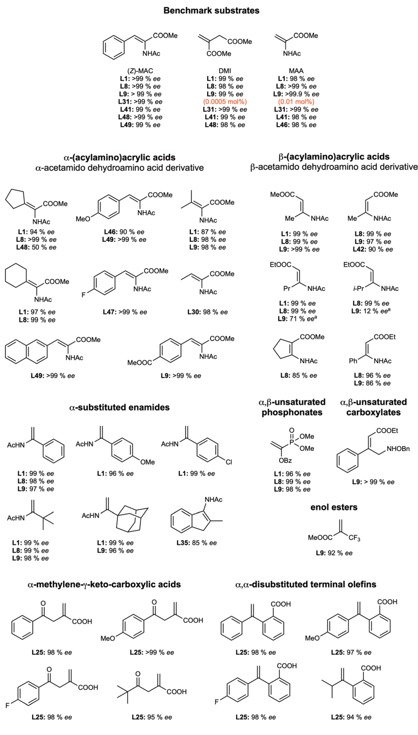
Fig. 5 Selected substrates used in Rh-catalysed enantioselective hydrogenation with PCP ligands and their corresponding enantioselectivities. a (Z)-isomer.
