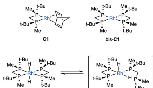
Fig. 4 Monochelated complex (C1) bischelated complex (bis-C1) (top). Equilibrium between the observed dihydrogenated species and the proposed hemilabile intermediate (bottom). Counter anions ( \text{PF}_6^- or \text{BF}_4^- ) have been omitted for clarity.
