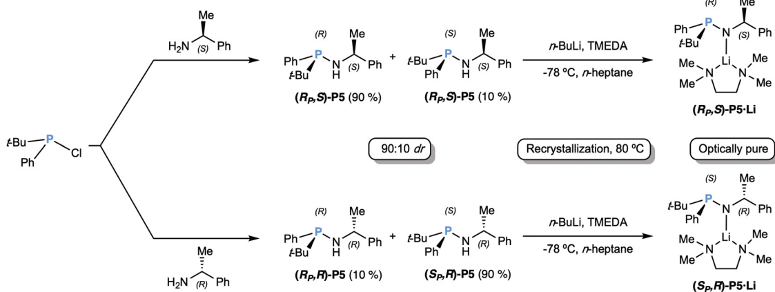
Scheme 34 Preparation of both enantiomers of nucleophilic synthon P5-Li .
