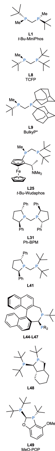
Fig. 5 Selected substrates used in Rh-catalysed enantioselective hydrogenation with PCP ligands and their corresponding enantioselectivities. a (Z)-isomer.
