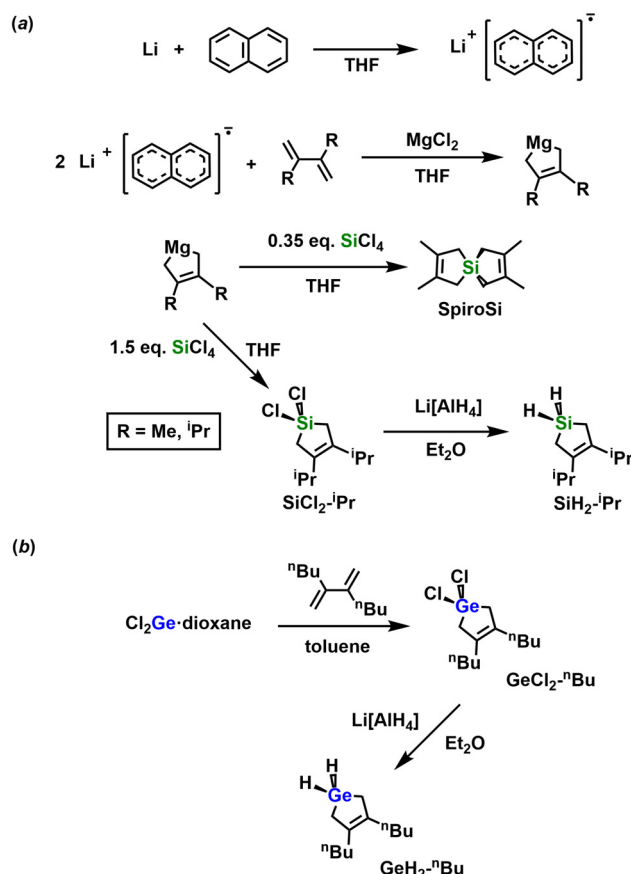
Scheme 1 (a) Synthesis of silaspiro-[4.4]-2,3,7,8-tetramethyl-2,7-nona-diene ( SpiroSi ) and 1,1-dihydro-3,4-di-iso-propylsilacyclopent-3-ene ( SiH 2 -iPr ); (b) synthesis of 1,1-dichloro-3,4-dibutylgermacyclopent-3-ene GeCl 2 - n Bu and 1,1-dihydro-3,4-dibutylgermacyclopent-3-ene GeH 2 - n Bu .
