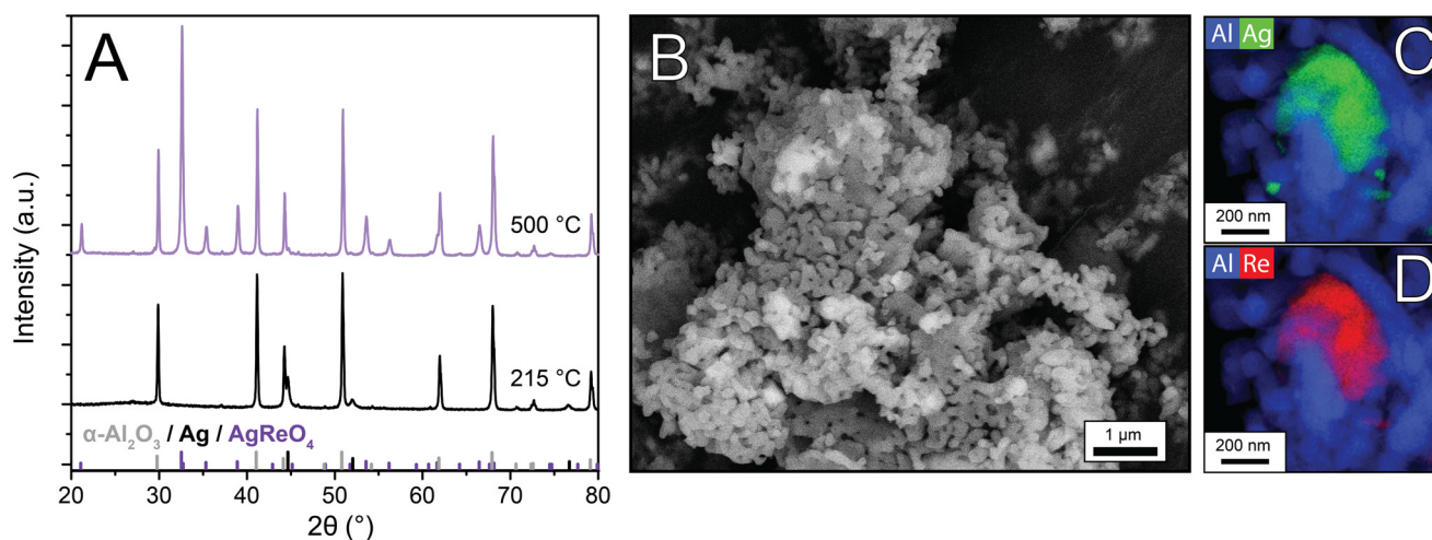
Fig. 4 X-ray diffractograms of the \text{AgReO}_4 samples calcined at 215 and 500^\circ\text{C} , with theoretical stick diffraction patterns of \alpha - \text{Al}_2\text{O}_3 , Ag and \text{AgReO}_4 below (A), SEM image of \text{AgReO}_4/\alpha - \text{Al}_2\text{O}_3 calcined at 500^\circ\text{C} (B) and STEM-EDX maps of a zoomed \text{AgReO}_4/\alpha - \text{Al}_2\text{O}_3 particle (C and D).
