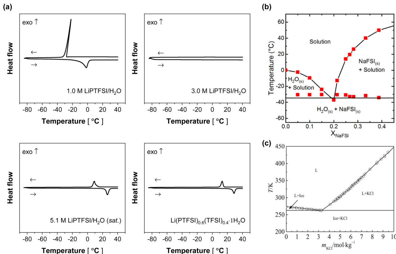
Fig. 19 (a) Thermal stability of LiPTFSI-based aqueous electrolytes evaluated by differential scanning calorimetry at a rate of 5^\circ\text{C min}^{-1} . 85 Phase diagrams of (b) NaFSI-H 2 O 89 and (c) KCl-H 2 O binary systems. 231 Reprinted with permission from Electrochemistry Communications (a), ACS Materials Letters (b), and Calphad (c).
