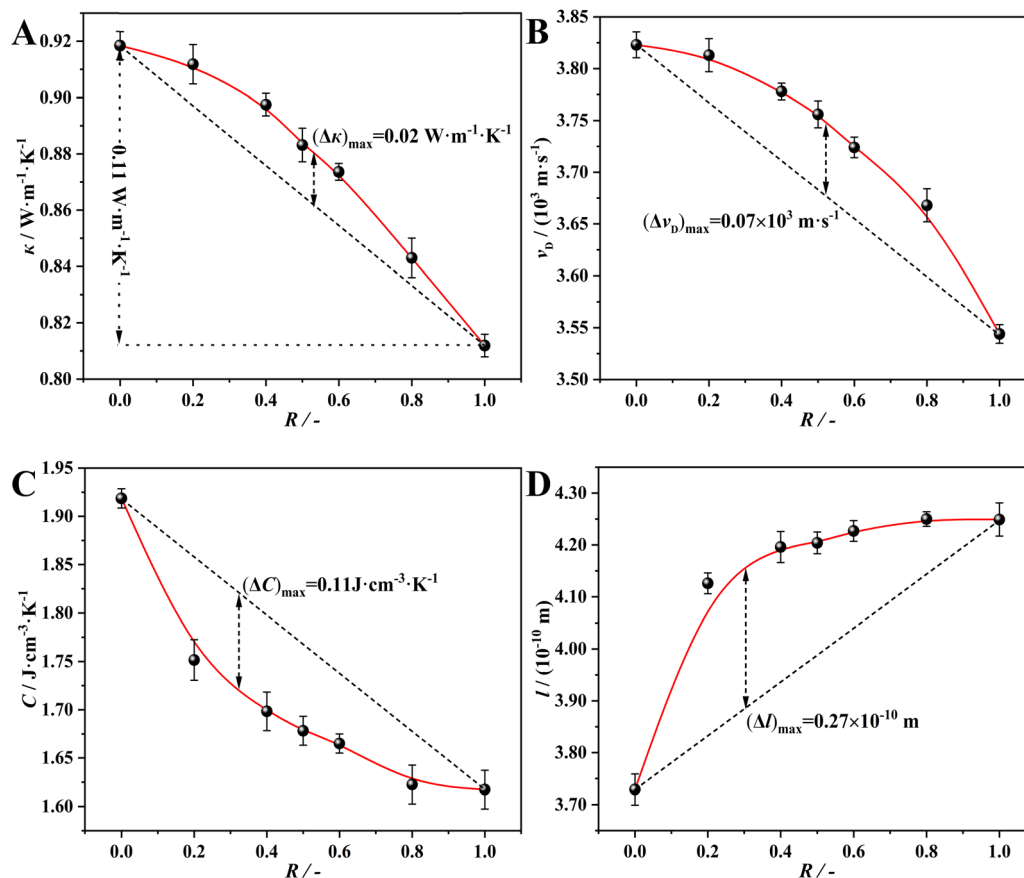
Fig. 2 Compositional dependence of (A) thermal conductivity ( \kappa ) and (C) volumetric heat capacity ( C ) at room temperature of the 65.0\text{SiO}_2\cdot 5.0\text{B}_2\text{O}_3 ( 17.6 - x )- \text{Na}_2\text{O}\cdot x\text{K}_2\text{O}\cdot 7.5\text{CaO}\cdot 4.9\text{MgO} glasses as a function of different molar ratios R , where R is equal to the molar ratio of [\text{K}_2\text{O}]/([\text{Na}_2\text{O}] + [\text{K}_2\text{O}]) . (B) Debye sound velocity ( \nu_D ) at room temperature plotted as a function of different molar ratios R . (D) Compositional dependence of the phonon mean free path ( l ) on R . Dashed line: the linear correlation between the two endmembers.
