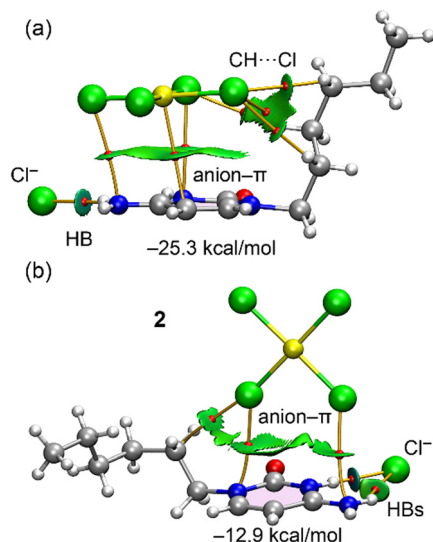
Fig. 11 Combined QTAIM (BCPs as red spheres and bond paths as orange lines) and NCIPLOT (RDG = 0.5, \rho cut-off = 0.04, color scale \pm 0.035 a.u.) for parallel (a) and T-shape (b) anion- \pi binding modes. Only intermolecular interactions are represented.
