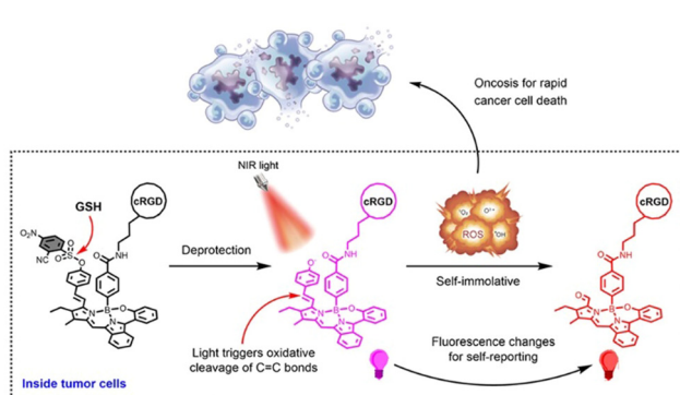
Fig. 3 Photooxidative cleavage of C=C bonds as an effective strategy to develop self-reporting self-immolative photosensitizers in cancer cells. Figure adapted from ref. 23 Copyright: 2023, with the permission from American Chemical Society.
