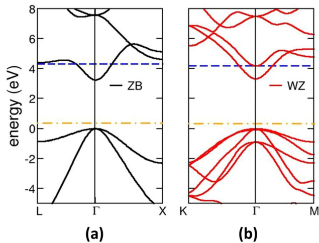
Fig. 6 Band structures of the two forms of ZnS: (a) zinc blende and (b) wurtzite.
