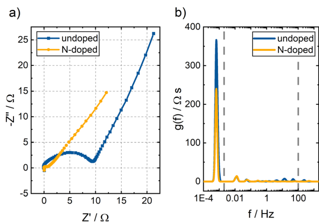
Fig. 7 (a) Nyquist plots and (b) DRT spectra of undoped and N-doped BC. A V(\text{IV}) electrolyte and a flow rate of 15 mL \text{min}^{-1} were used. A potential of 1.05 V vs. RHE was applied.
