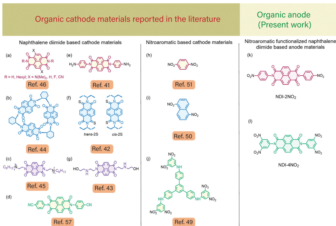
Fig. 1 Various cathodes reported in the literature (corresponding specific capacity and average potential V vs. \text{Li}^+/\text{Li} ). (a) N -hexyl-nitrile-substituted NDI 9 ( 105\text{ mA h g}^{-1}@0.2\text{C} , 2.8 V), (b) (–)-NDI- \Delta ( 150\text{ mA h g}^{-1}@0.1\text{C} , 2.5 V), (c) NDI-rGO ( 200\text{ mA h g}^{-1}@25\text{ mA g}^{-1} , 2.4 V), (d) NDI-CN, (e) naphthalenediimide diamine ( 240\text{ mA h g}^{-1}@50\text{ mA g}^{-1} , 2.1 V), (f) P-NDI trans -2S and cis -2S ( 120\text{ mA h g}^{-1}@50\text{ mA g}^{-1} , 2.40 V), (g) NDI-NHOH ( 122\text{ mA h g}^{-1}@0.05\text{C} , 2.36 V), (h) p -DNB ( 535\text{ mA h g}^{-1}@50\text{ mA g}^{-1} , 2.67 V), (i) 1,5-DNN ( 1338\text{ mA h g}^{-1}@20\text{ mA g}^{-1} , 2.45 V), and (j) TAPB-6NO 2 ( 120\text{ mA h g}^{-1}@50\text{ mA g}^{-1} , 2.0 V). (a)–(g) Naphthalene diimide-based small molecules as cathode materials, (h)–(j) nitroaromatic compounds as cathode materials, and (k) and (l) nitroaromatic functionalized NDIs as anode materials reported in the present work.
